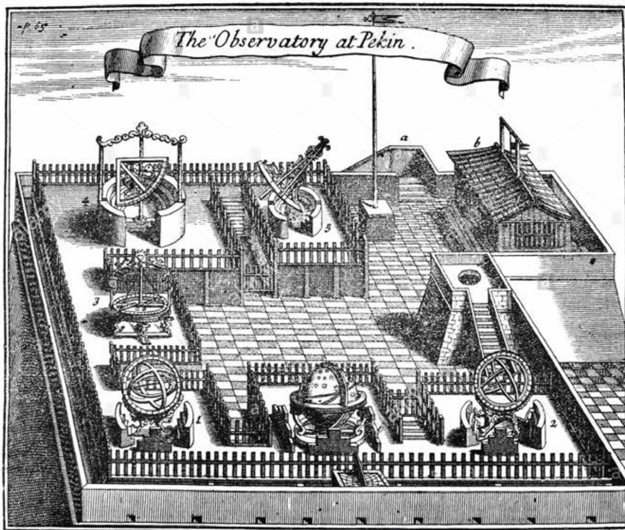
a. Steps going up to the Observatory | 1. a Zodiacal Sphere | 3. an Azimuthal Horizon | 5. A Sextant b. A Retiring Room for those that make Observations | 2. an Equinoctial Sphere | 4. a Quadrant | 6. a Celestial Globe
